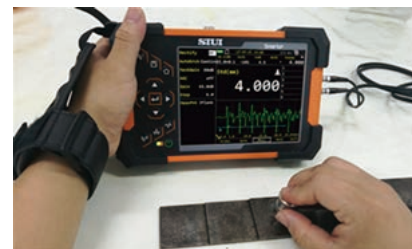
● Thickness measurement on step block
