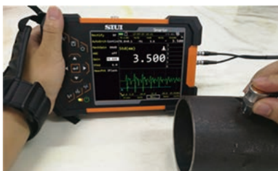
● Thickness measurement on pipe
