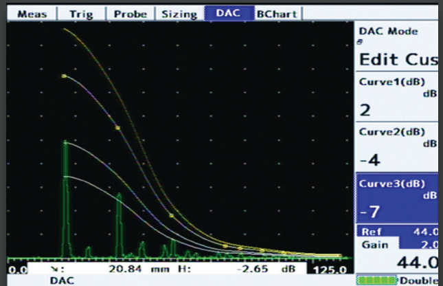
Customisable DAC
