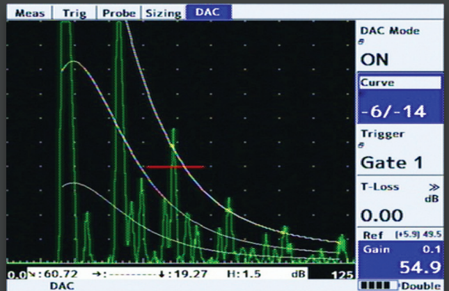
Dynamic DAC
